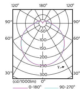
LEDtube 100mm 5W G24D-1
