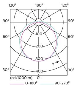
LEDtube PLC 100mm 9W G24D-3 865 1000lm
