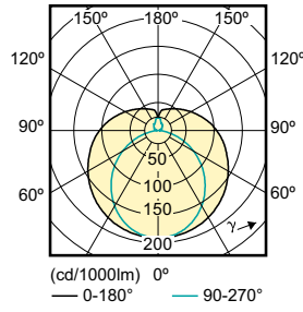
LEDtube 1200mm 18 W T8 C W G
