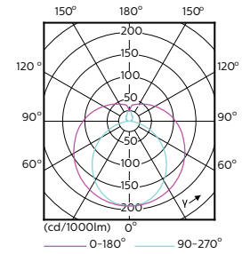
LEDtube 1500mm 20W G13 840 2200lm
