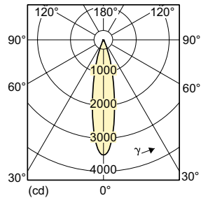
12.5 W E26 3000 K PAR30S 25D
