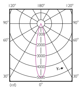
PAR30S 12W 950lm 25D 2700K E26
