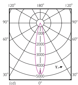
PAR30S 12W 850lm 25D 2700K E26
