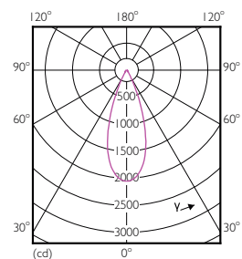
PAR30S 12W 850lm 40D 2700K E26
