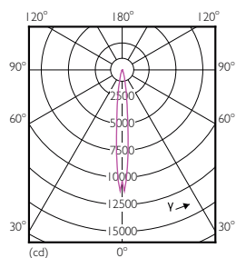
PAR30S 12W 850lm 10D 2700K E26
