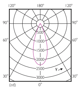
PAR30S 12W 950lm 40D 2700K E26
