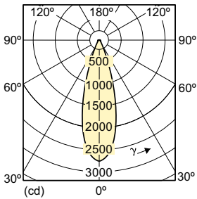
12 W E26 3500 K PAR30S 36D
