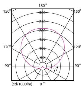
LEDbulb 120W E27 827 FR A67
