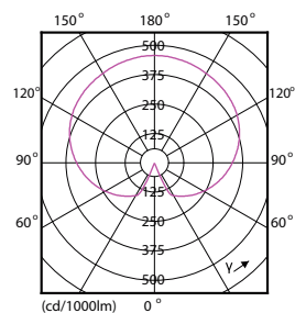
CorePro LEDbulb 40W B22 827 FR A60
