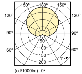
6.5-48 W /830 3000K 220-240V
