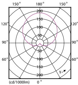
CorePro LEDbulb 75W B22 827 FR A60
