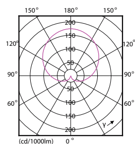
CorePro LEDbulb 100W E27 840 FR A60
