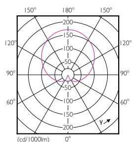
CorePro LEDbulb 40W E27 830 FR A60
