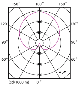
CorePro LEDbulb 60W B22 827 FR A60
