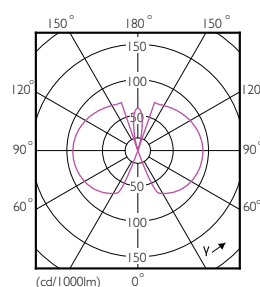
Bulb G25 120V 500lm 150D WW E26 ND
