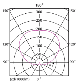
CorePro LEDbulb 100W B22 827 FR A67
